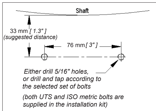
Figure 3 : Mounting holes for the synchronization probe
