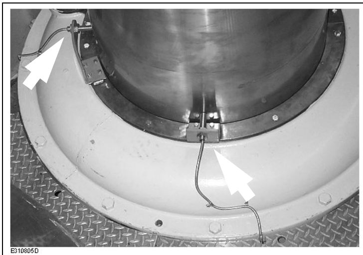
Figure 6 : Two PCS-200SB sensors installed for radial vibration measurement
