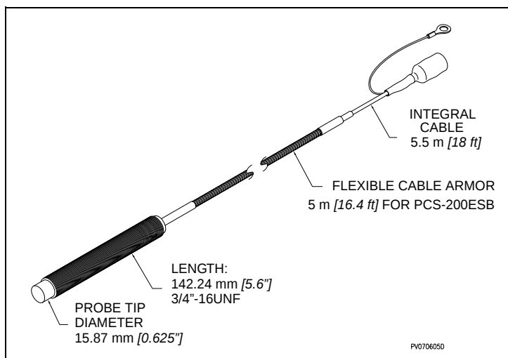
Figure 4 : Legacy PCS-200ESB sensor terminated with BNC connector
