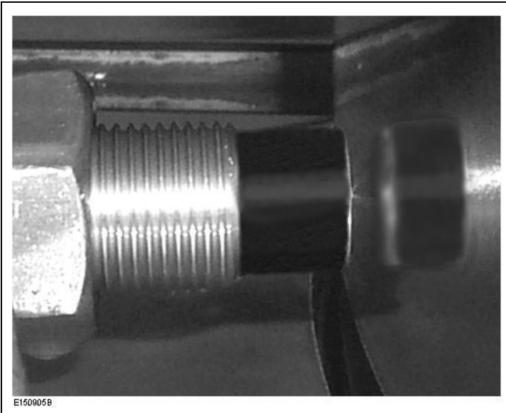
Figure 7 : Sensor installed at mid-range distance from the target
