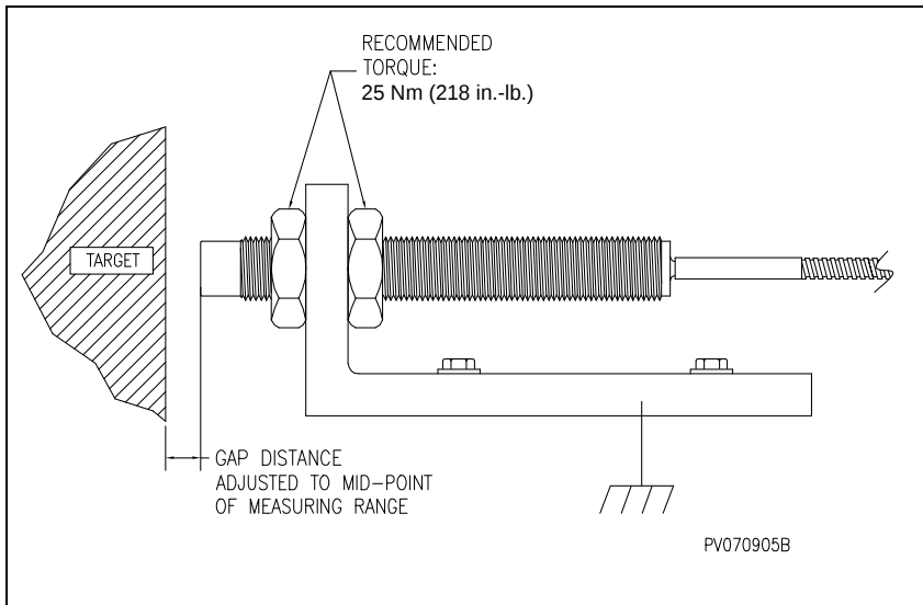
Figure 9 : Setting the PCS-200ESB sensor in place
