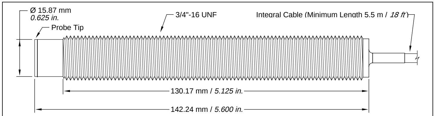
Figure 12 : PCS-200ESB dimensions
