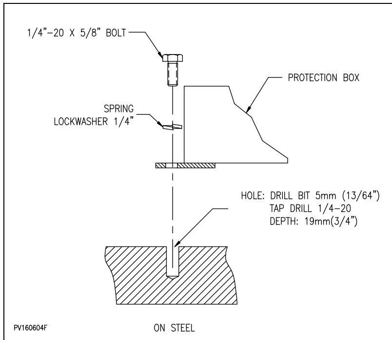
Figure 18 : Fastening the protection box on steel
