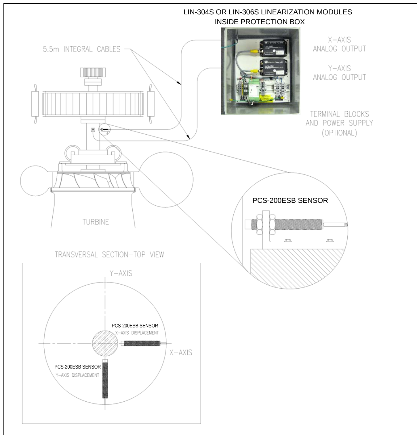
Figure 1 : Typical PCS-200ESB / LIN-300 Series measuring chains installation
