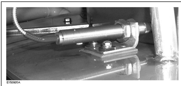
Figure 3 : PCS-200ESB Sensor installed on a bracket
