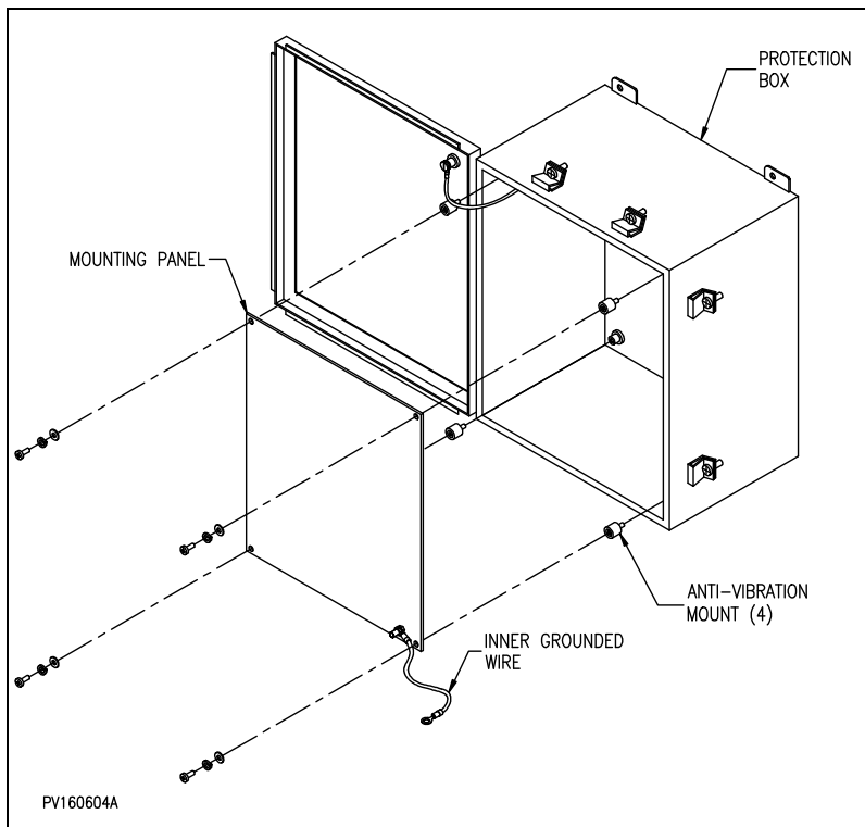
Figure 13 : Removing the mounting panel and anti-vibration mounts
